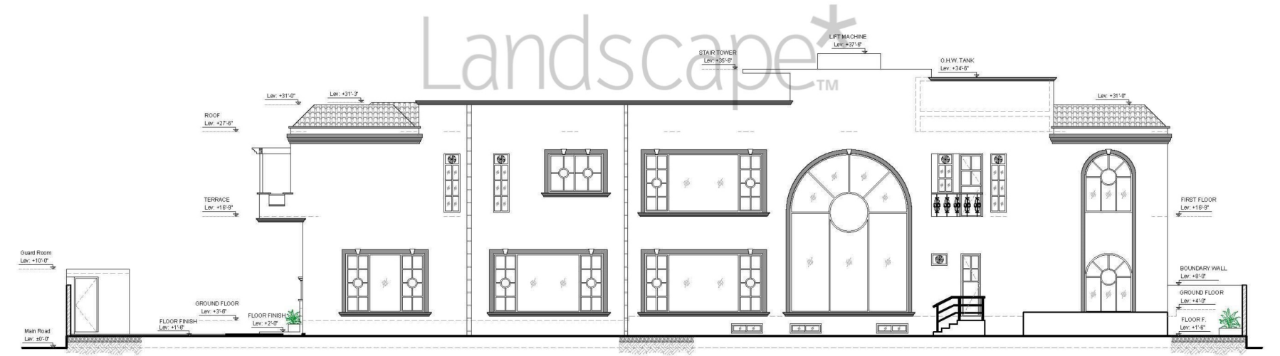
LEFT ELEVATION
