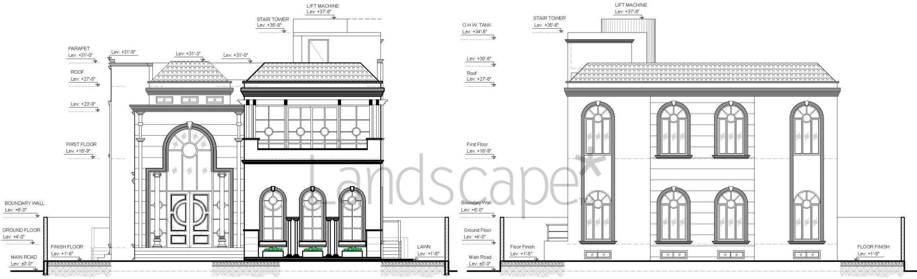
FRONT ELEVATION
